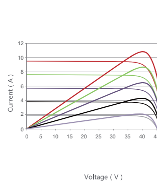
Current-Voltage & Power-Voltage Curves (370W)
