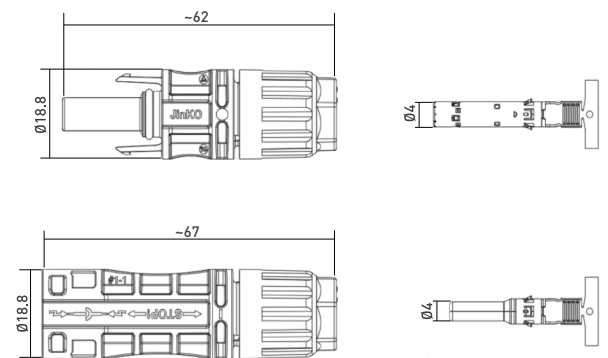
Female Housing
